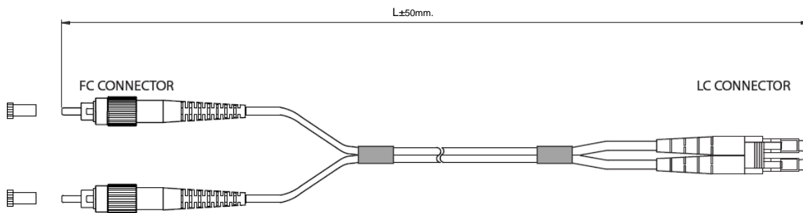
FC to LC FIBER OPTIC PATCH CORD
