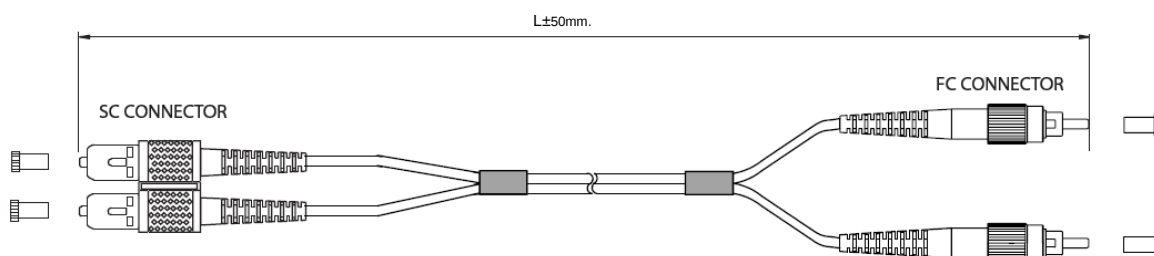
SC to FC FIBER OPTIC PATCH CORD
