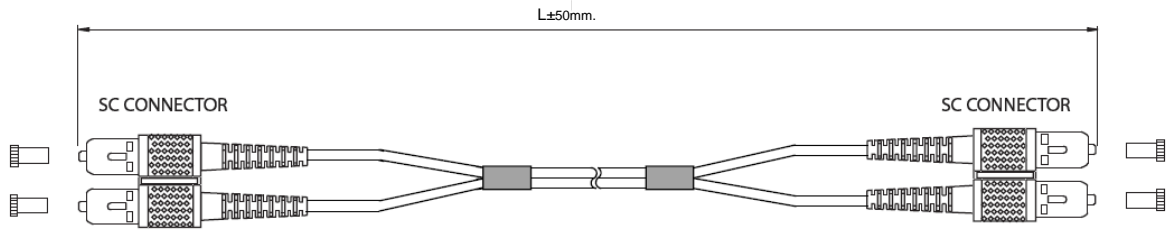
SC to SC FIBER OPTIC PATCH CORD
