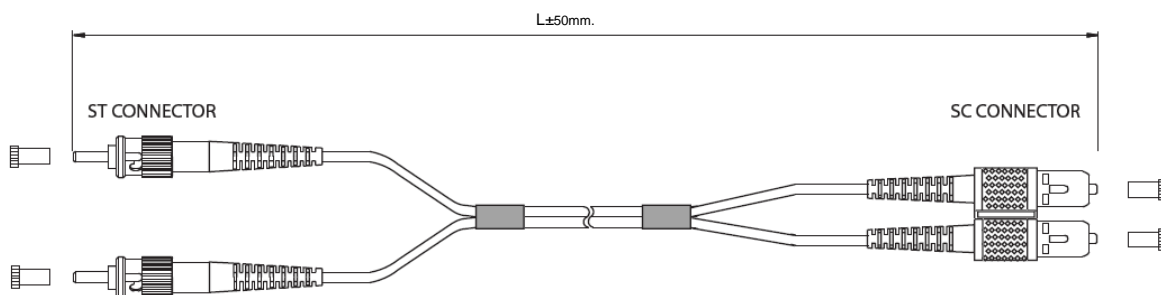
ST to SC FIBER OPTIC PATCH CORD
