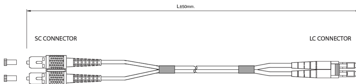
SC to LC FIBER OPTIC PATCH CORD
