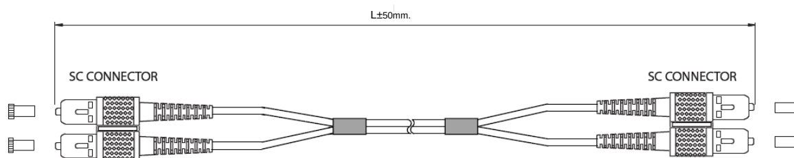
SC to SC FIBER OPTIC PATCH CORD
