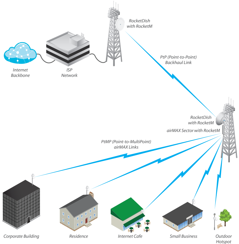
The RocketDish antennas paired with RocketM devices create a powerful PtP backhaul link.
